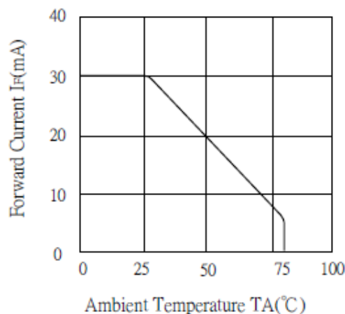
MAX FORWARD CURRENT Vs. AMBIENT TEMPERATURE
