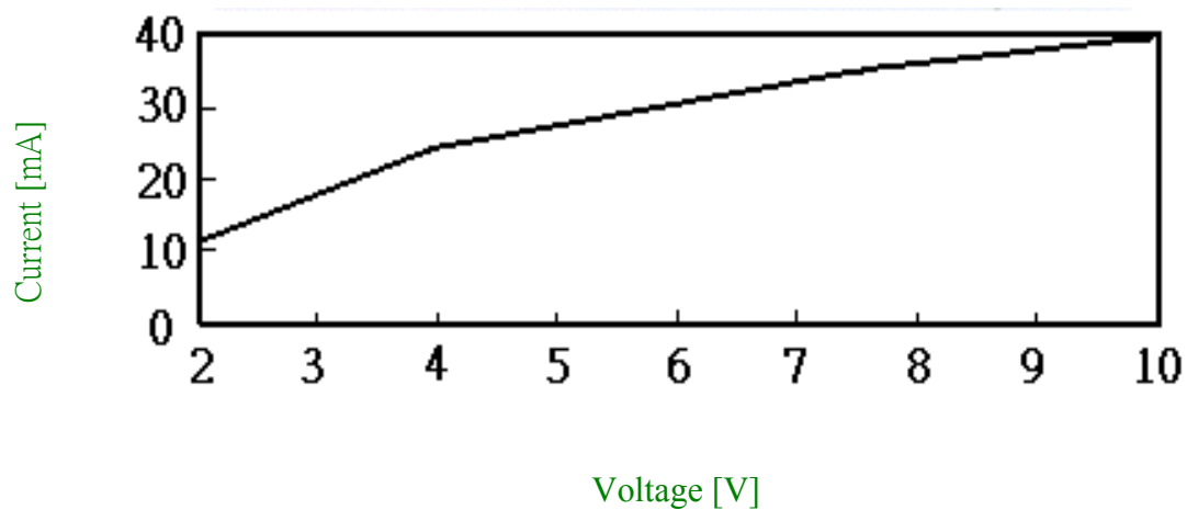
Source output current VS. Operating
