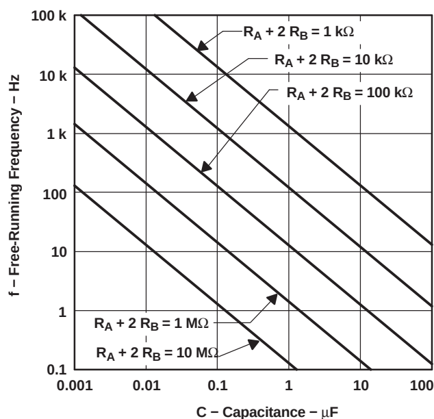
Figure 14. Free-Running Frequency
